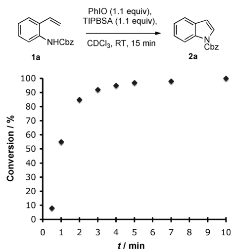
Figure 1. Kinetic profile for formation of indole 2a from 1a .
