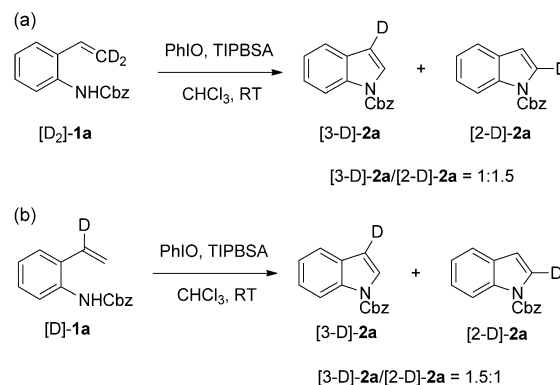
Scheme 4. Control experiments using selectively deuterated derivatives of 1a .
